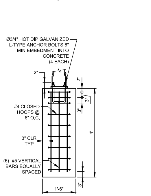
CONCRETE BASE
