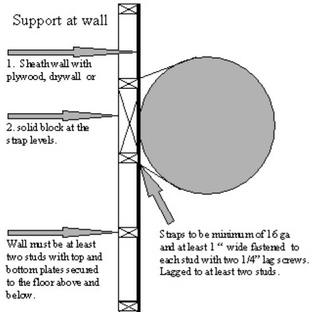
Plan View
